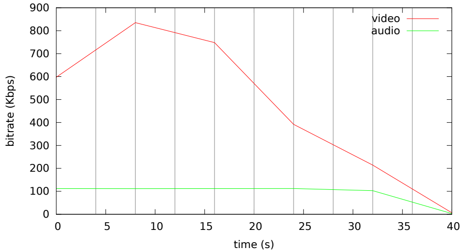
Bitrate analysis of videos-abr/motiongraphics-abr.mp4
