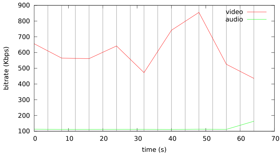
Bitrate analysis of videos-abr/fluidmotion-abr.mp4
