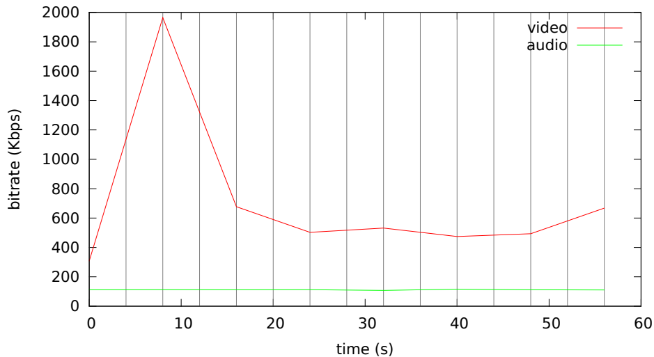
Bitrate analysis of videos-abr/presentation-abr.mp4
