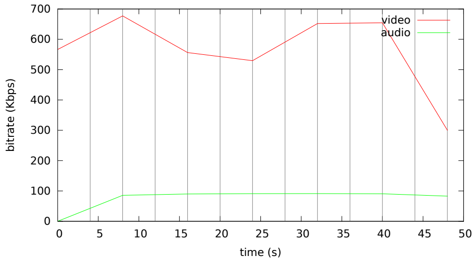
Bitrate analysis of videos-abr/interview-abr.mp4
