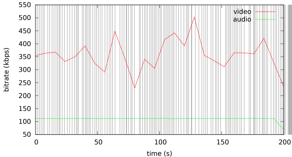
Bitrate analysis of videos-default4/blackwhite-default4.mp4
