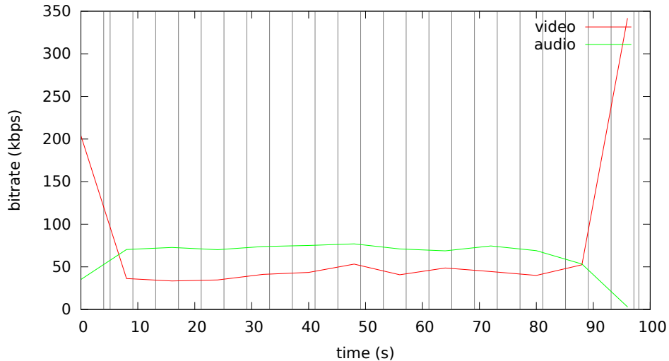
Bitrate analysis of videos-default4/screencast-default4.mp4
