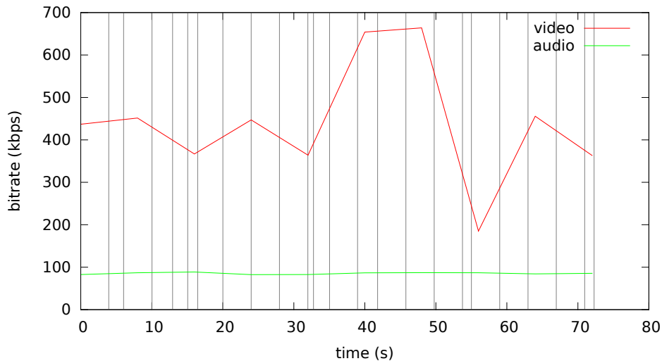
Bitrate analysis of videos-default4/soccer-default4.mp4
