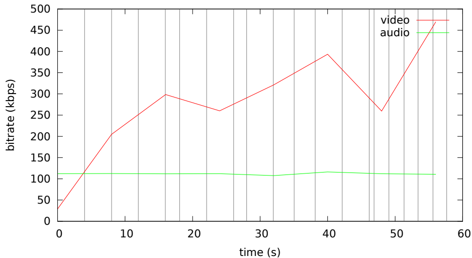
Bitrate analysis of videos-default4/presentation-default4.mp4
