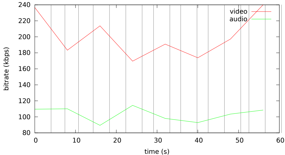
Bitrate analysis of videos-default4/crap-default4.mp4
