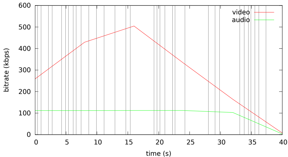
Bitrate analysis of videos-default4/motiongraphics-default4.mp4
