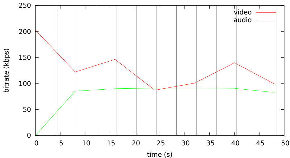
Bitrate analysis of videos-default4/interview-default4.mp4
