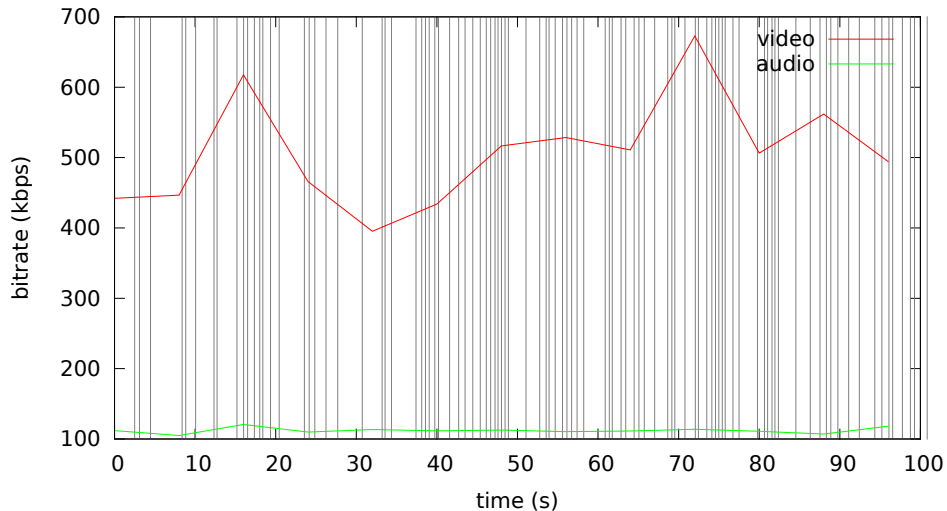
Bitrate analysis of videos-default4/movietrailer-default4.mp4
