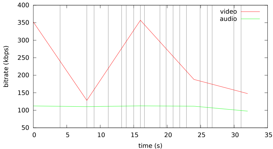
Bitrate analysis of videos-default4/animation-default4.mp4
