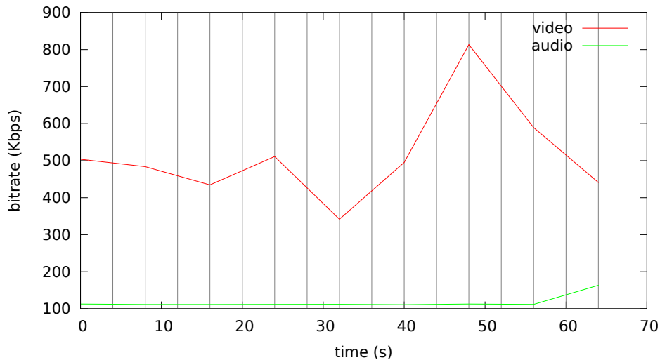
Bitrate analysis of videos-vbv3/fluidmotion-vbv3.mp4
