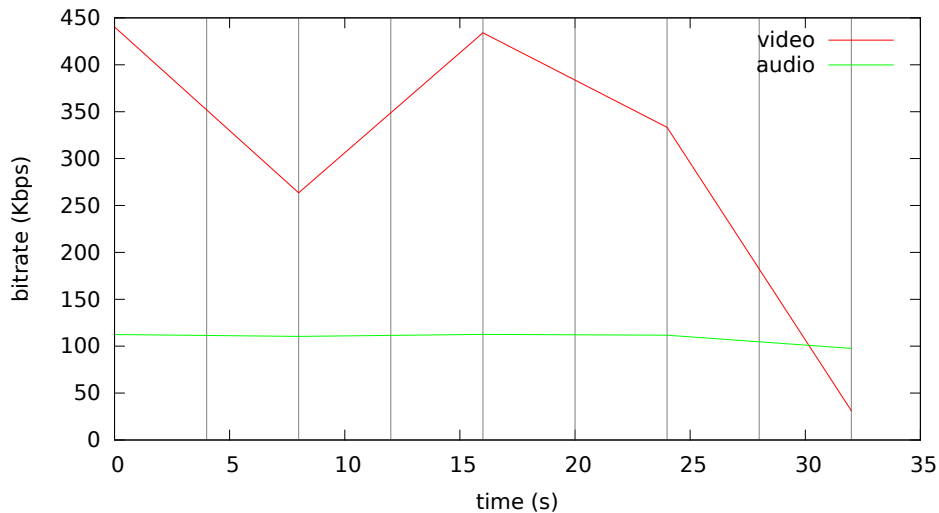
Bitrate analysis of videos-vbv3/animation-vbv3.mp4
