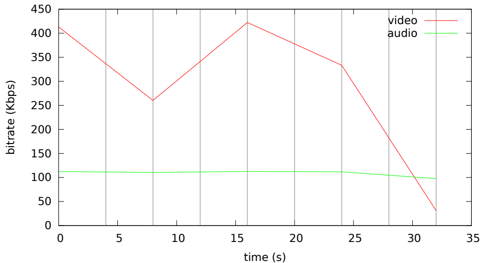
Bitrate analysis of videos-vbv4/animation-vbv4.mp4
