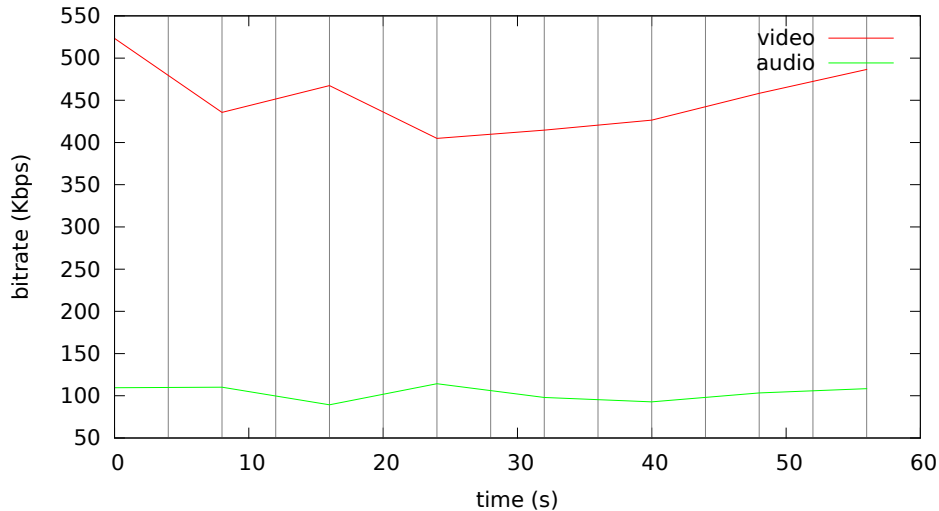
Bitrate analysis of videos-vbv4/crap-vbv4.mp4
