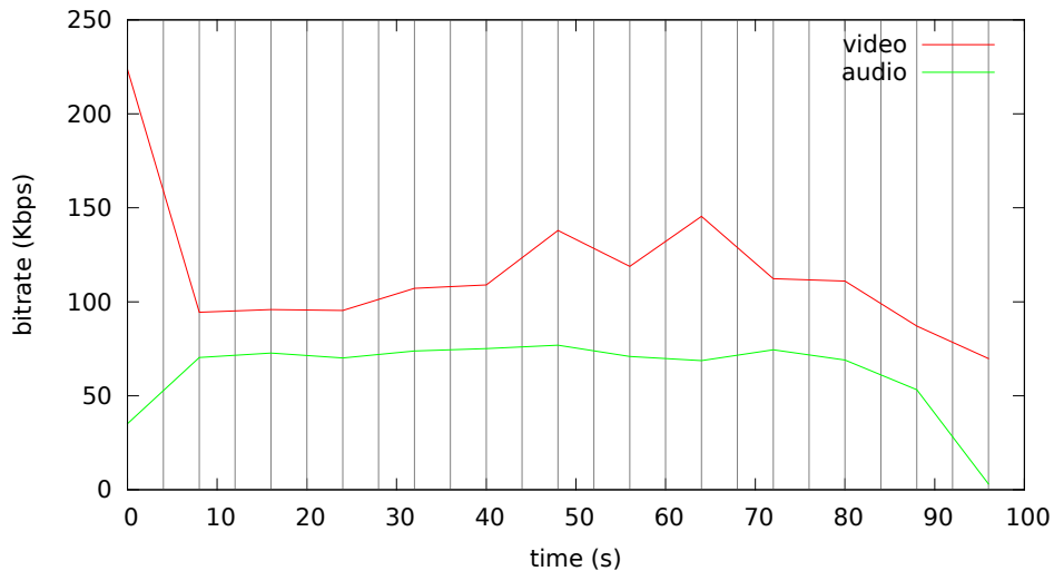
Bitrate analysis of videos-vbv4/screencast-vbv4.mp4
