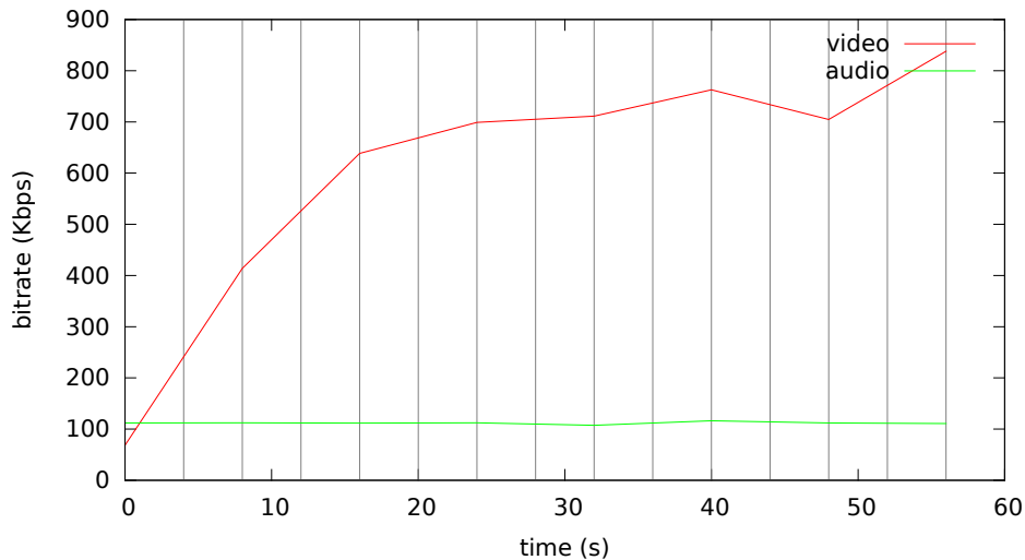
Bitrate analysis of videos-vbv4/presentation-vbv4.mp4
