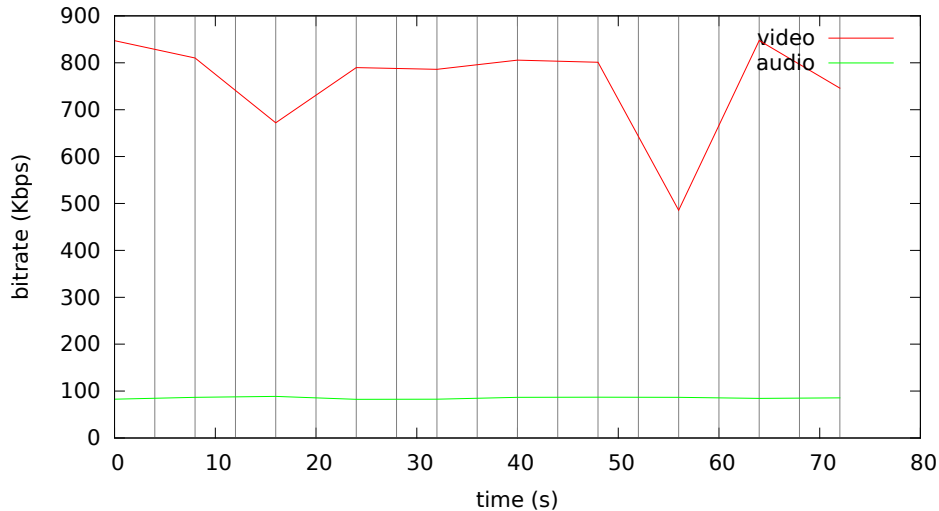
Bitrate analysis of videos-vbv4/soccer-vbv4.mp4
