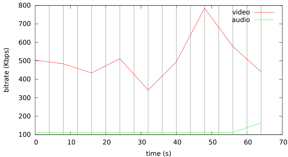
Bitrate analysis of videos-vbv4/fluidmotion-vbv4.mp4
