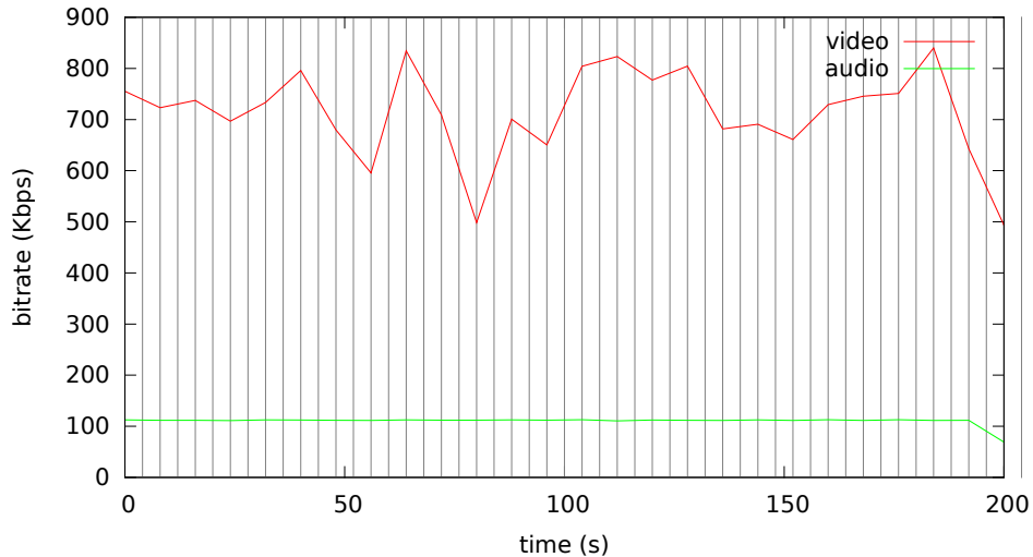
Bitrate analysis of videos-vbv4/blackwhite-vbv4.mp4
