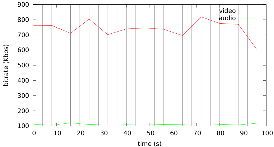
Bitrate analysis of videos-vbv4/movietrailer-vbv4.mp4
