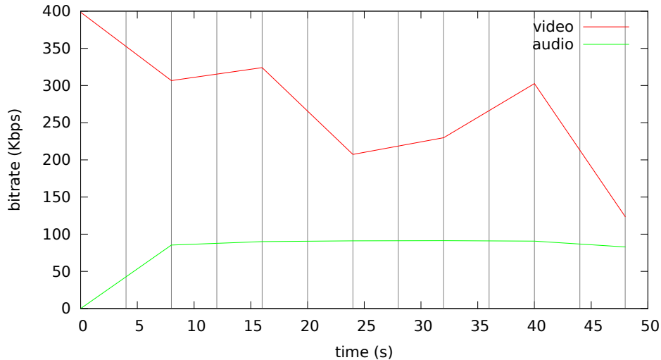
Bitrate analysis of videos-vbv4/interview-vbv4.mp4
