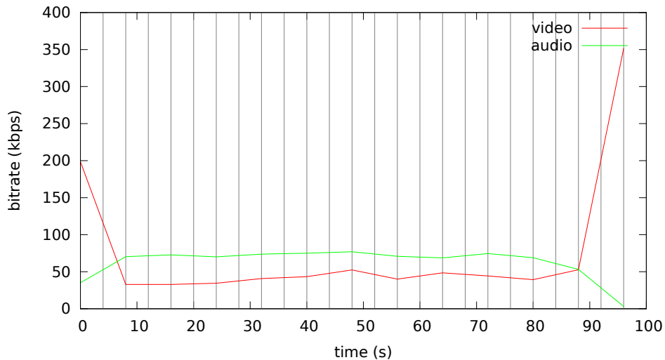
Bitrate analysis of videos-vbv41/screencast-vbv41.mp4
