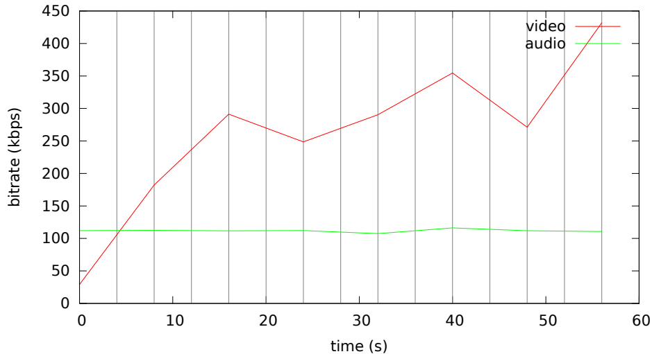
Bitrate analysis of videos-vbv41/presentation-vbv41.mp4
