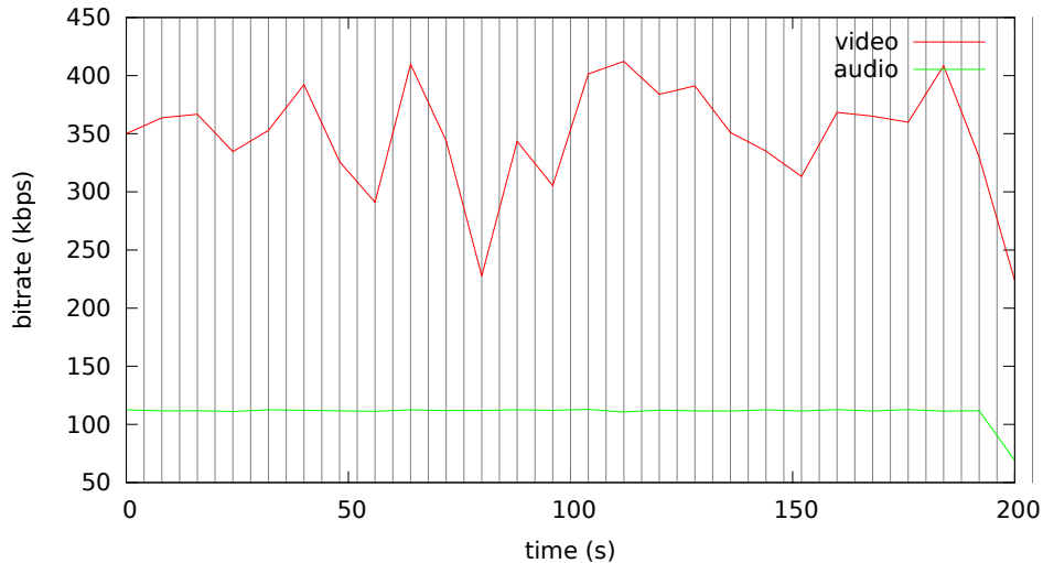
Bitrate analysis of videos-vbv41/blackwhite-vbv41.mp4
