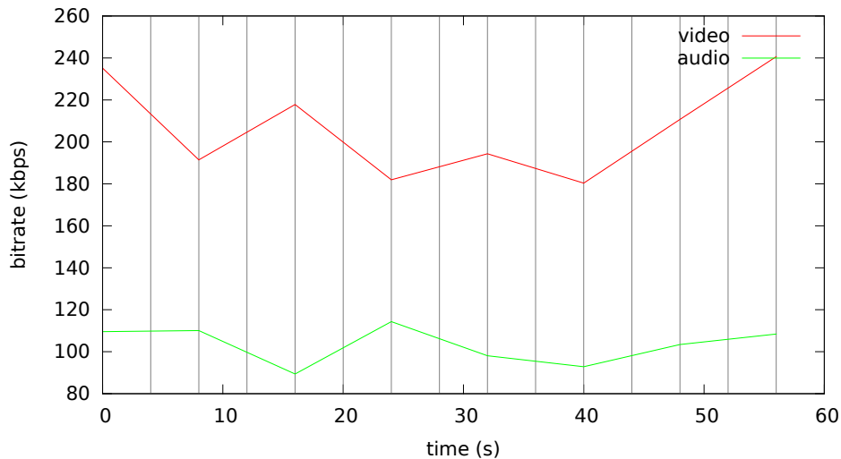
Bitrate analysis of videos-vbv41/crap-vbv41.mp4
