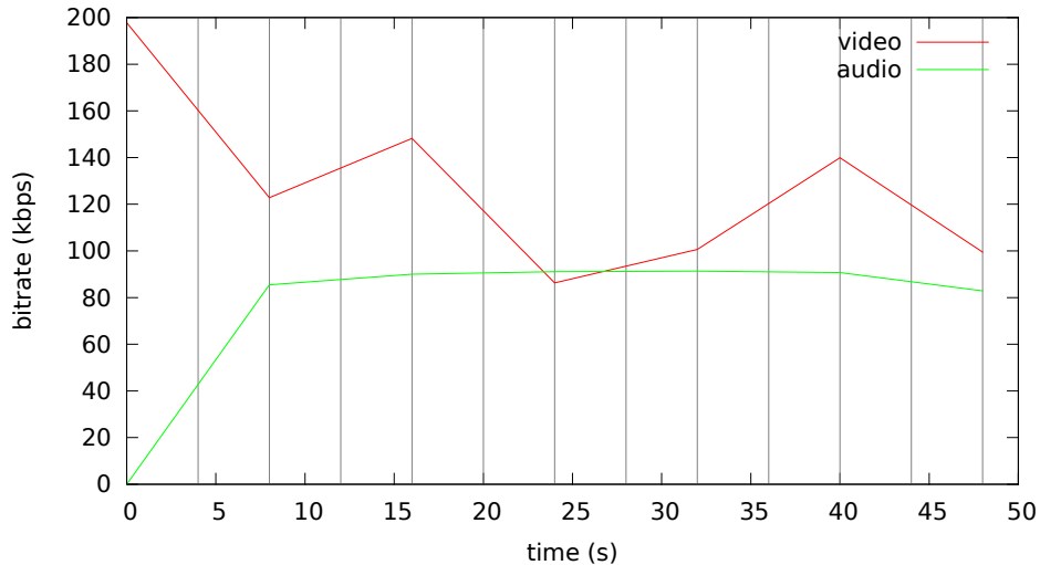
Bitrate analysis of videos-vbv41/interview-vbv41.mp4
