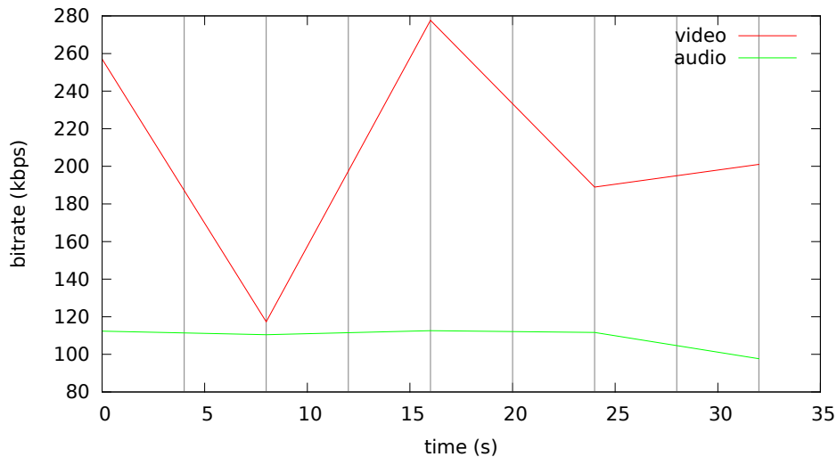
Bitrate analysis of videos-vbv41/animation-vbv41.mp4
