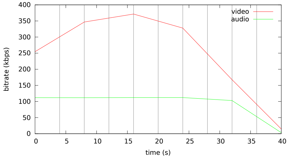
Bitrate analysis of videos-vbv41/motiongraphics-vbv41.mp4
