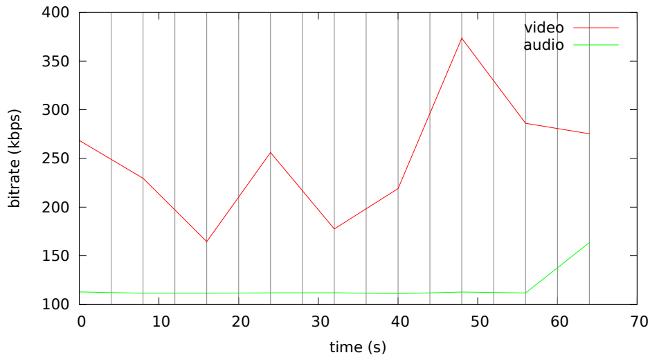
Bitrate analysis of videos-vbv41/fluidmotion-vbv41.mp4
