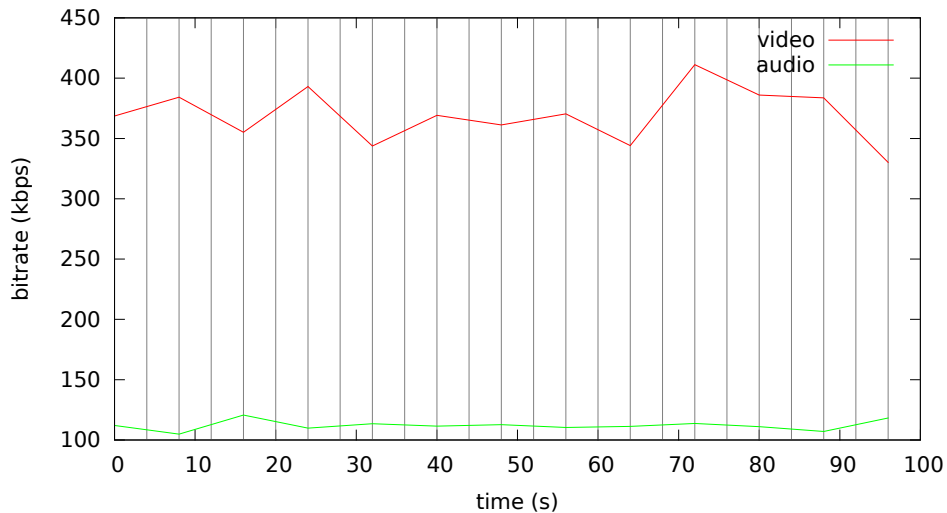
Bitrate analysis of videos-vbv41/movietrailer-vbv41.mp4
